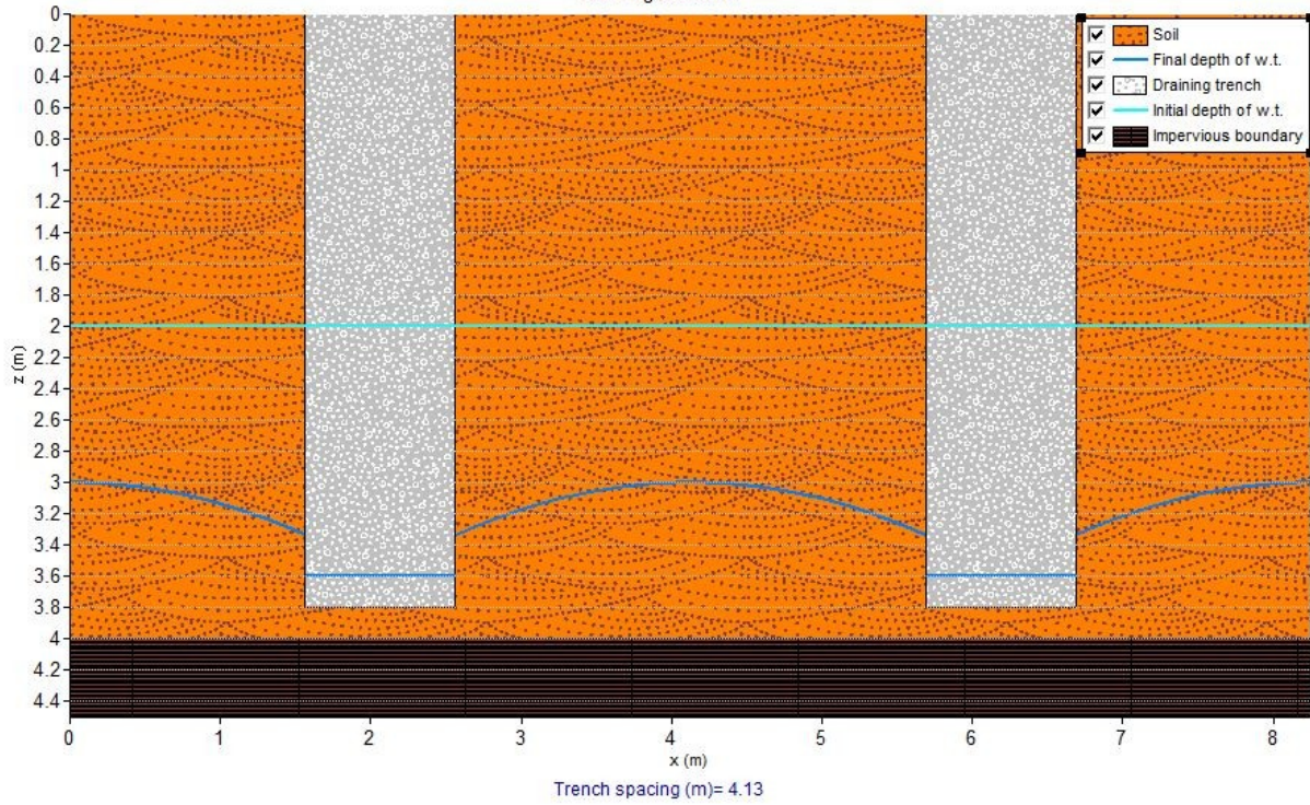
Draining trenches
