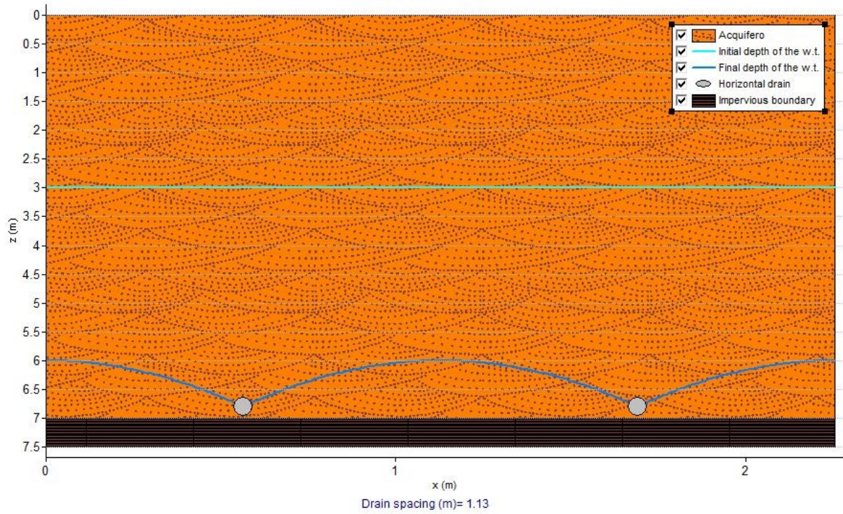
Horizontal drain scheme
