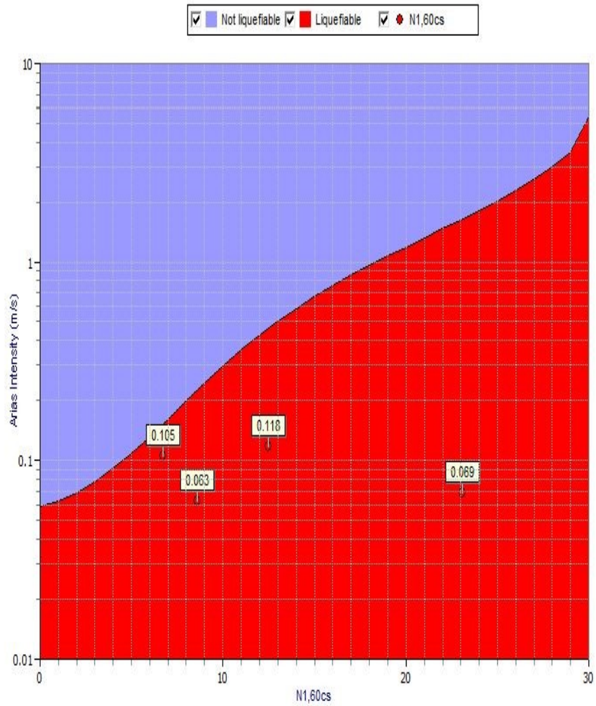
Liquefaction by Arias Intensity (Kayen e Mitchell, 1997)
